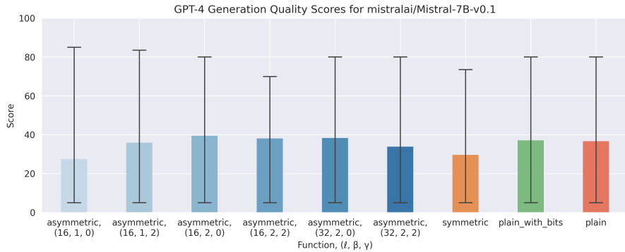
Figure 2: Aggregated text quality score assignments from GPT-4 Turbo for each generation algorithm configuration over the Mistral 7B model [JSM + 23]. For asymmetric , the configurations from left to right represent the most compact (lowest quality) to least compact (highest quality) parameters. Each bar is the aggregation of GPT-4 Turbo-assigned quality scores for 250 distinct prompt completions. The error bars show the 95% interval data spread. Observe that no protocol clearly outperforms the others: the mean score falls between 27 and 40 for all protocols, and each one exhibits large quality spreads. Note that even the baseline decoder, plain , follows this pattern. This suggests the watermarking protocols are indeed distortion-free.
