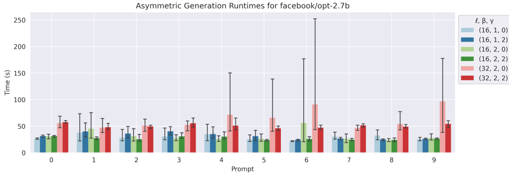
Figure 4: Generation runtimes for each variant of our protocol over the OPT-2.7B model [ZRG + 22]. Generation runtimes for different parameter instantiations of our protocol. 5 completions were generated for each of the 10 random prompts from the news-like portion of the C4 dataset [RSR + 20]. \ell denotes the signature segment length, \beta denotes the bit size, and \gamma denotes the maximum number of planted errors. The error bars show the 95% interval data spread. Comparing non-error-corrected ( \gamma = 0 ) vs. error-corrected ( \gamma = 2 ) runtimes for prompts with high variance (prompts 4, 5, 6, 8, and 9 for parameters \ell = 32 , \beta = 2 and \ell = 16 , \beta = 2 ), we can see a clear reduction in the variance and mean runtime when error correction is applied to overcome low entropy periods. Note that we expect to sample E_\lambda(\ell, \beta) = 2^\beta \cdot \frac{\lambda}{\beta} \cdot \ell characters to embed the signature codeword. Thus, in expectation, E_\lambda(16, 1) = E_\lambda(16, 2) < E_\lambda(32, 2) where \lambda = 328 or 360 depending on if \gamma = 0 or 2 . Our empirical runtimes align with this.
