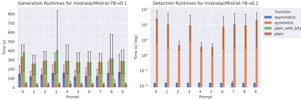
Figure 3: Generation and detection runtimes for each generation algorithm over the Mistral 7B model [JSM + 23]. Five distinct generations were aggregated for each of the 10 random prompts from the news-like portion of the C4 dataset [RSR + 20]. The error bars show the 95% interval data spread. On average, the fastest to slowest generation runtimes were for: plain (expected as this is the baseline), asymmetric , then symmetric and plain with bits (the latter two are about equal with the dominant cost being the reduction to a binary vocabulary). For detection, asymmetric runs much faster than symmetric which is expected given they run in linear vs. quadratic time, respectively, in the number of tokens n .
