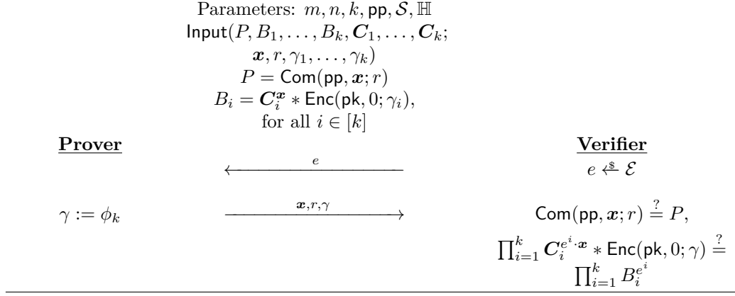
Figure 5 Compression Mechanism \Pi_C for relation \mathcal{R}_{\Psi}
